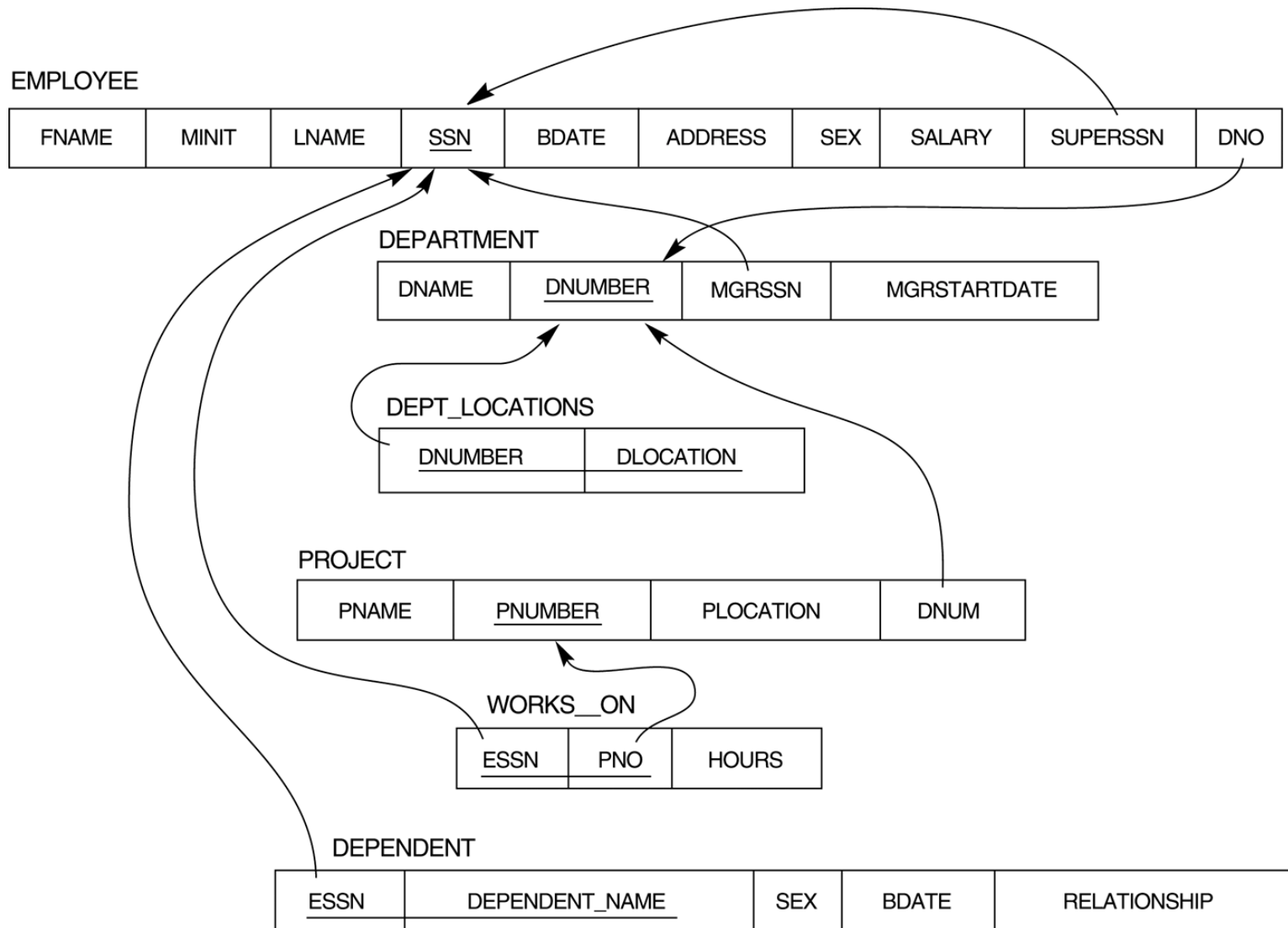
FIGURE: Result of mapping the COMPANY ER schema into a relational schema.
